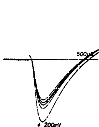
FIGURE 5 Time-course of decline of peak sodium current as observed with infrequent depolarizing pulses (dashed line) and of the further decline caused by repetitive stimulation as indicated. 1.3 \times 10^{-4} M external yohimbine.
