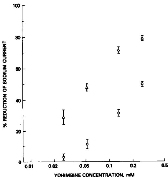
FIGURE 8 Dose-response curves for internal yohimbine. (○) Tonic effect. (△) Use-dependent effect. For use-dependent effect, pulse potential is 0 mV, pulse duration is 2 ms, and pulse frequency is 1 Hz.
